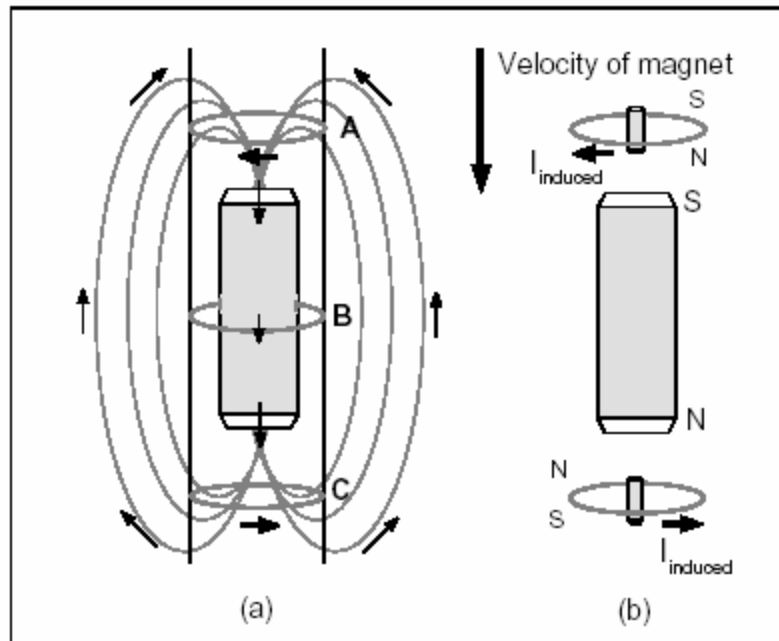
Figure 2 Diagram of the Falling Magnet
